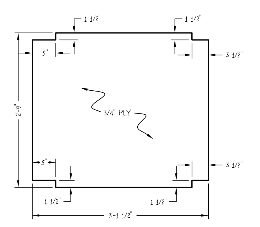
BOTTOM DETAIL SKIN BUILD THREE
