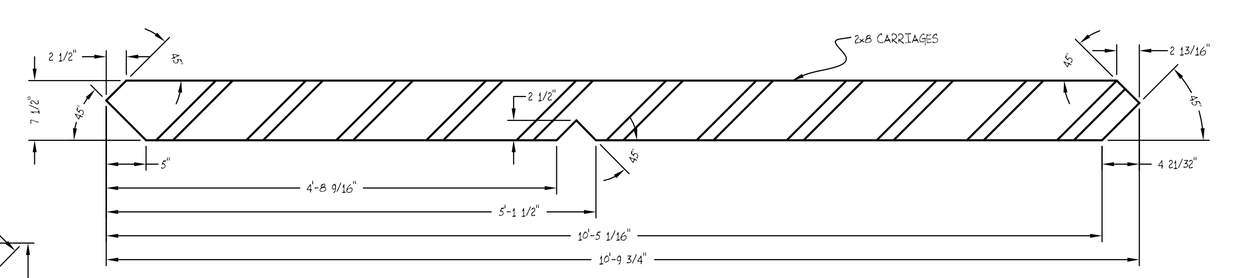
CARRIAGE LAYOUT 1 of 2
