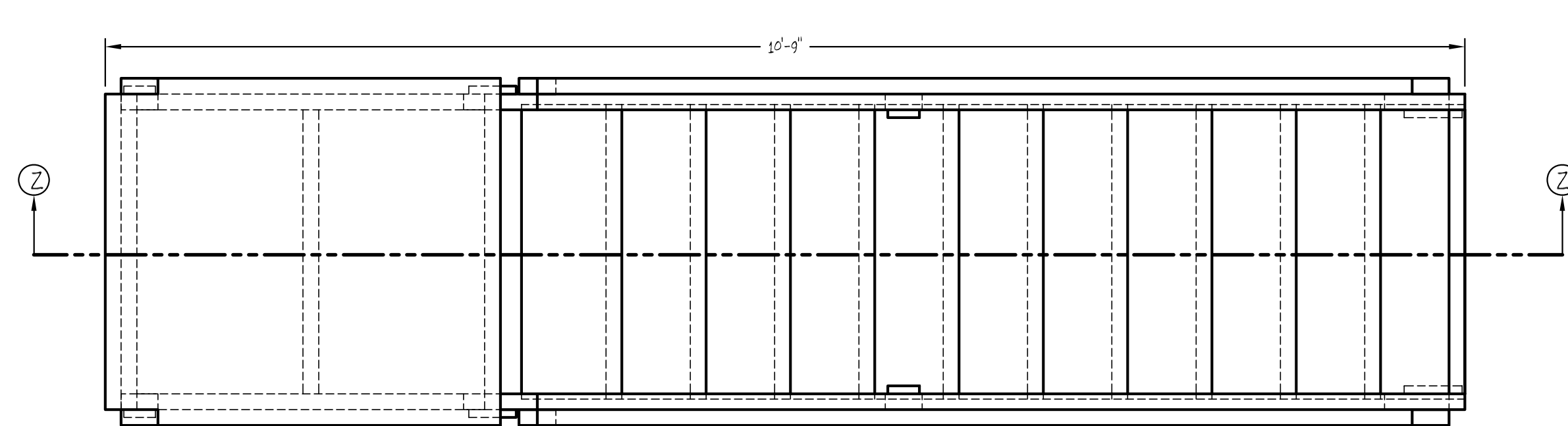
ESCAPE STAIR UNIT TOP, LIPTJACK REMOVED BUILD THREE
