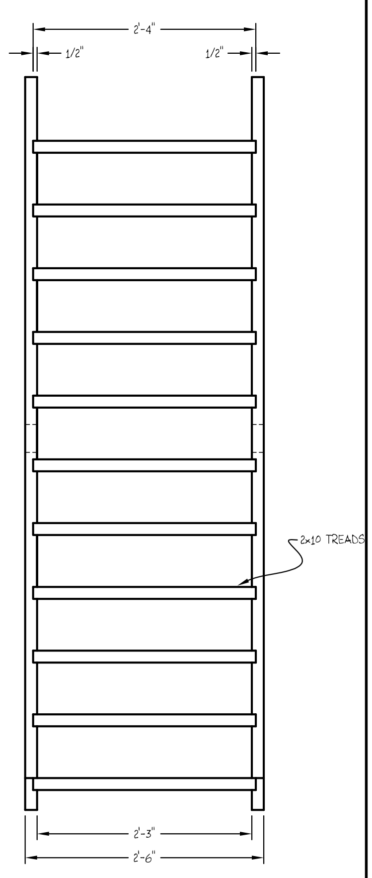
ESCAPE STAIRCASE BUILD THREE
