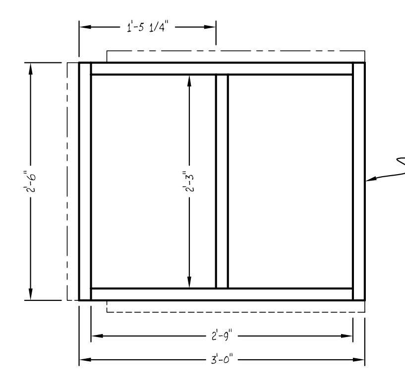
TOP DETAIL FRAMING BUILD THREE
