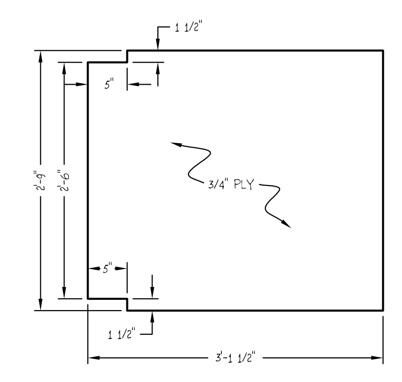
TOP DETAIL SKIN BUILD THREE
