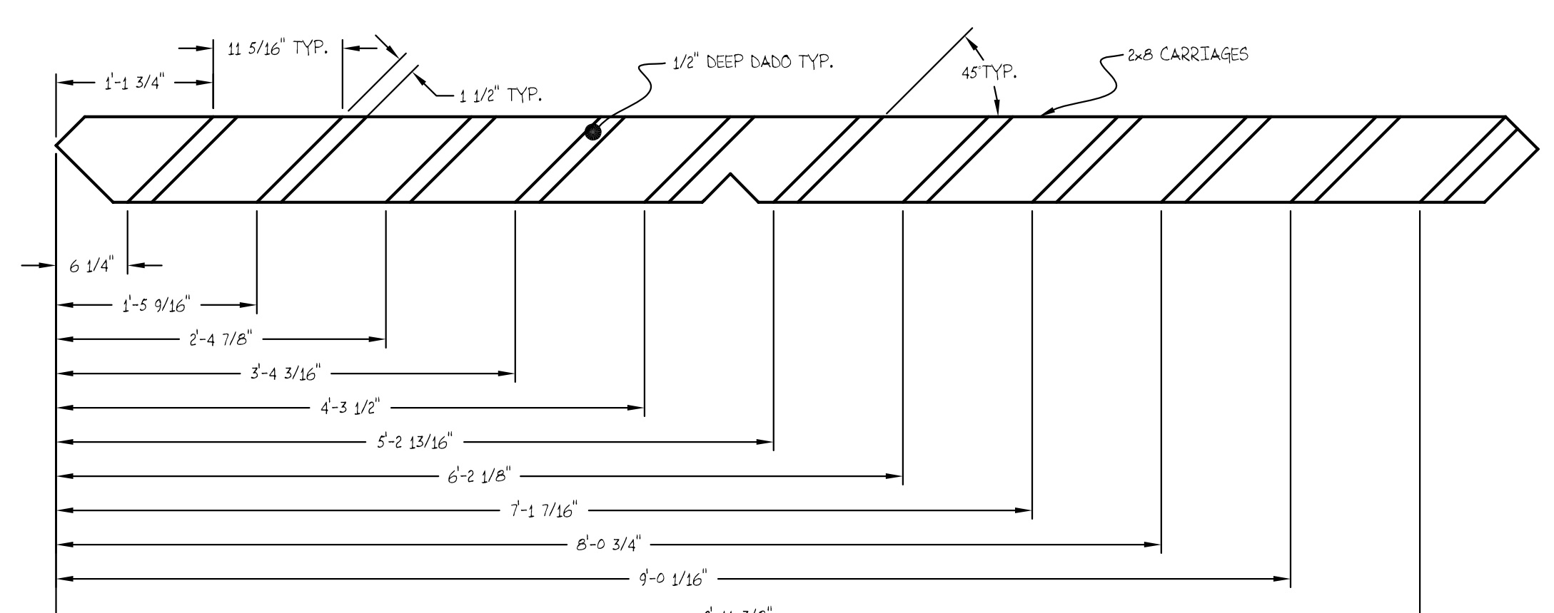
CARRIAGE LAYOUT 2 of 2
