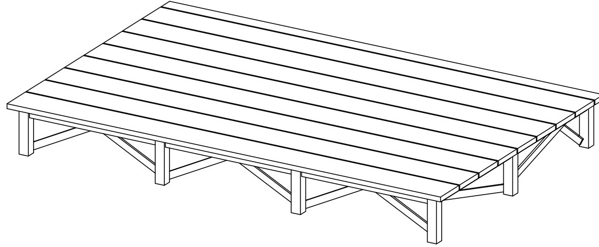
Platform 115 Assembled 3D View
